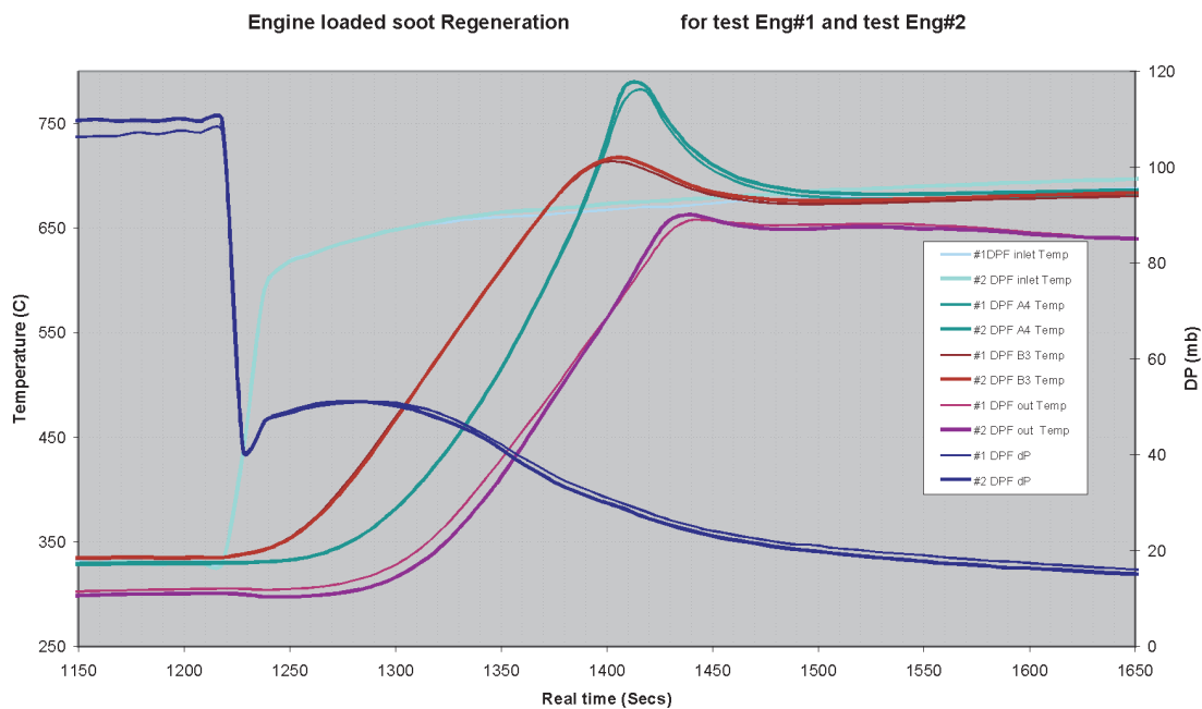
Fig. 8. Repeat of regeneration of ~32 g of Engine loaded soot
