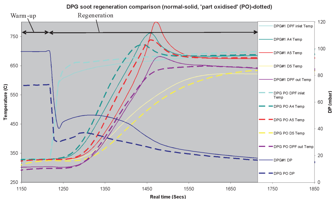
Fig. 12. Regeneration of normal DPG soot and part-oxidized (PO) DPG soot
