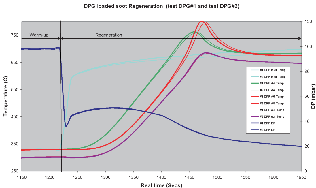
Fig. 7. Repeat of regeneration of ~32 g DPG soot
