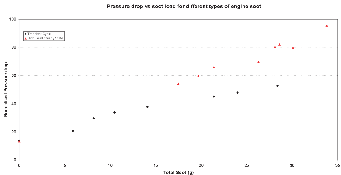
Fig. 10. DP vs sootlad for 2 types of Diesel engine soot
