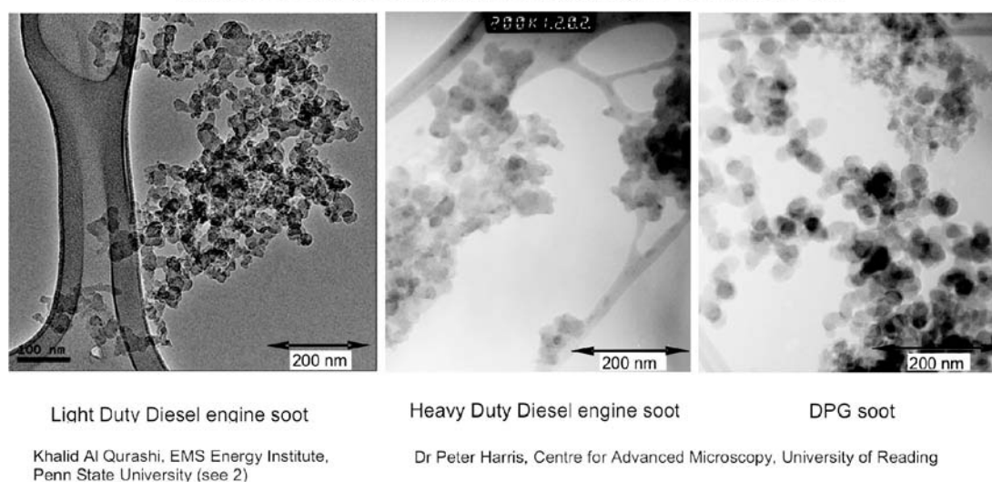
Fig. 11. TEM images of DPG soot and engine soot
