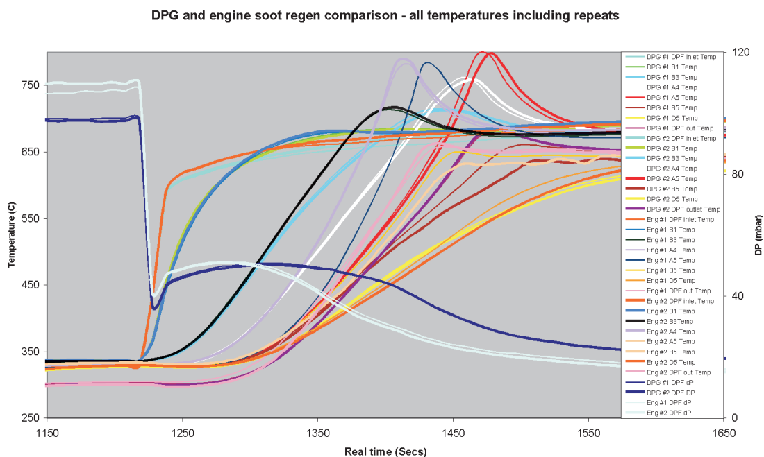
Fig. 6. Temperatures and pressure for all 4 regeneration tests
