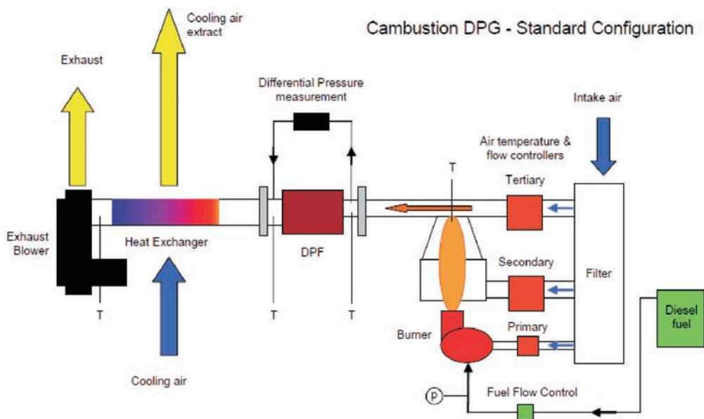
Fig. 1. DPG schematic description
