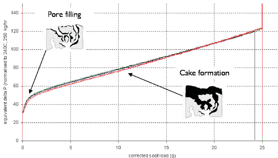
Fig. 4. Repeatability of soot load vs pressure drop for a standard DPF on uncoupled DPGs
