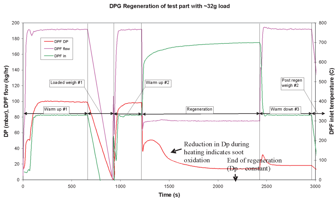
Fig. 5. Pressure drop, inlet temperature and flow during Regeneration schedule
