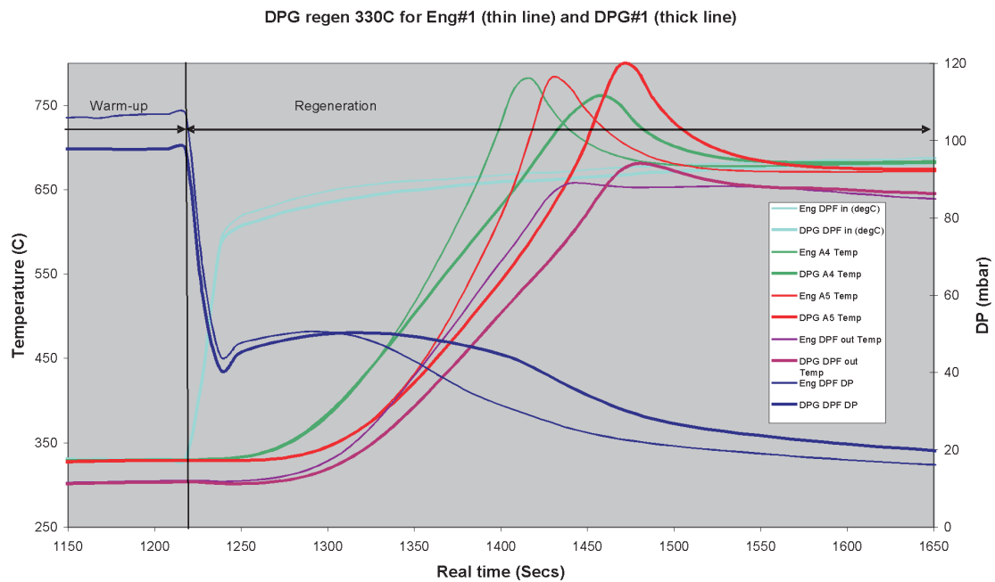
Fig. 9. Comparison of DPG and Engine loaded ~32 g soot regeneration
