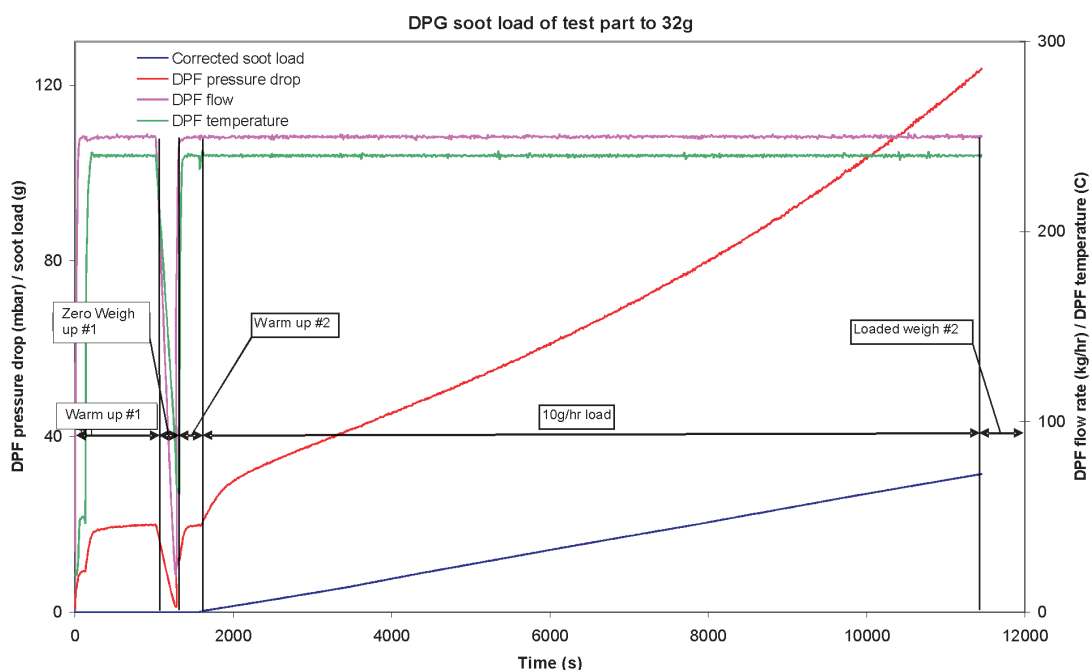
Fig. 3. Pressure drop across DPF, gas flow rate and inlet temperature during loading schedule
