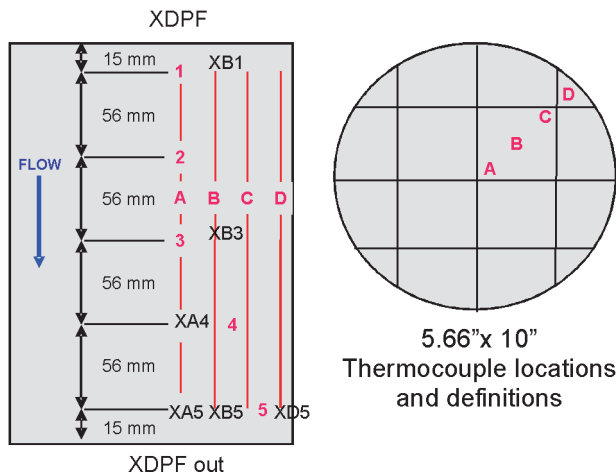
Fig. 2. Thermocouple locations in DPF
